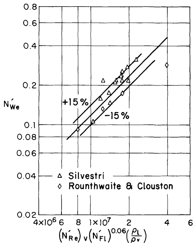
Fig. 13. Upper transition region data for water.
