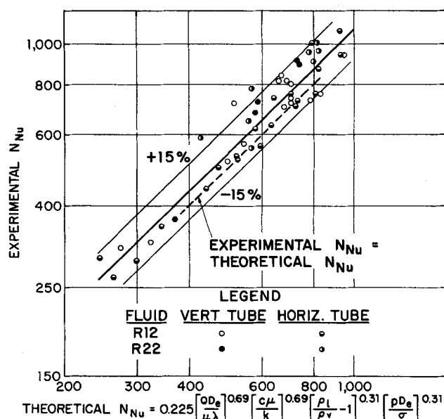
Fig. 5. Nucleate boiling correlation for plain tube.
