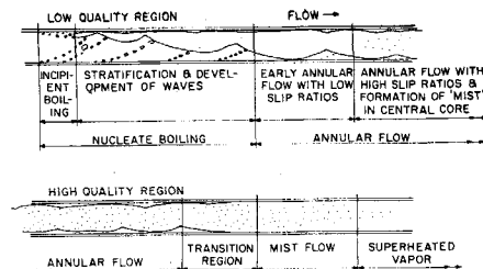
Fig. 4. Model of process of evaporation inside a horizontal tube.
